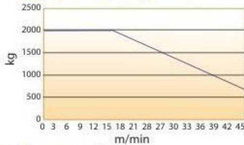
Speed Diagram
